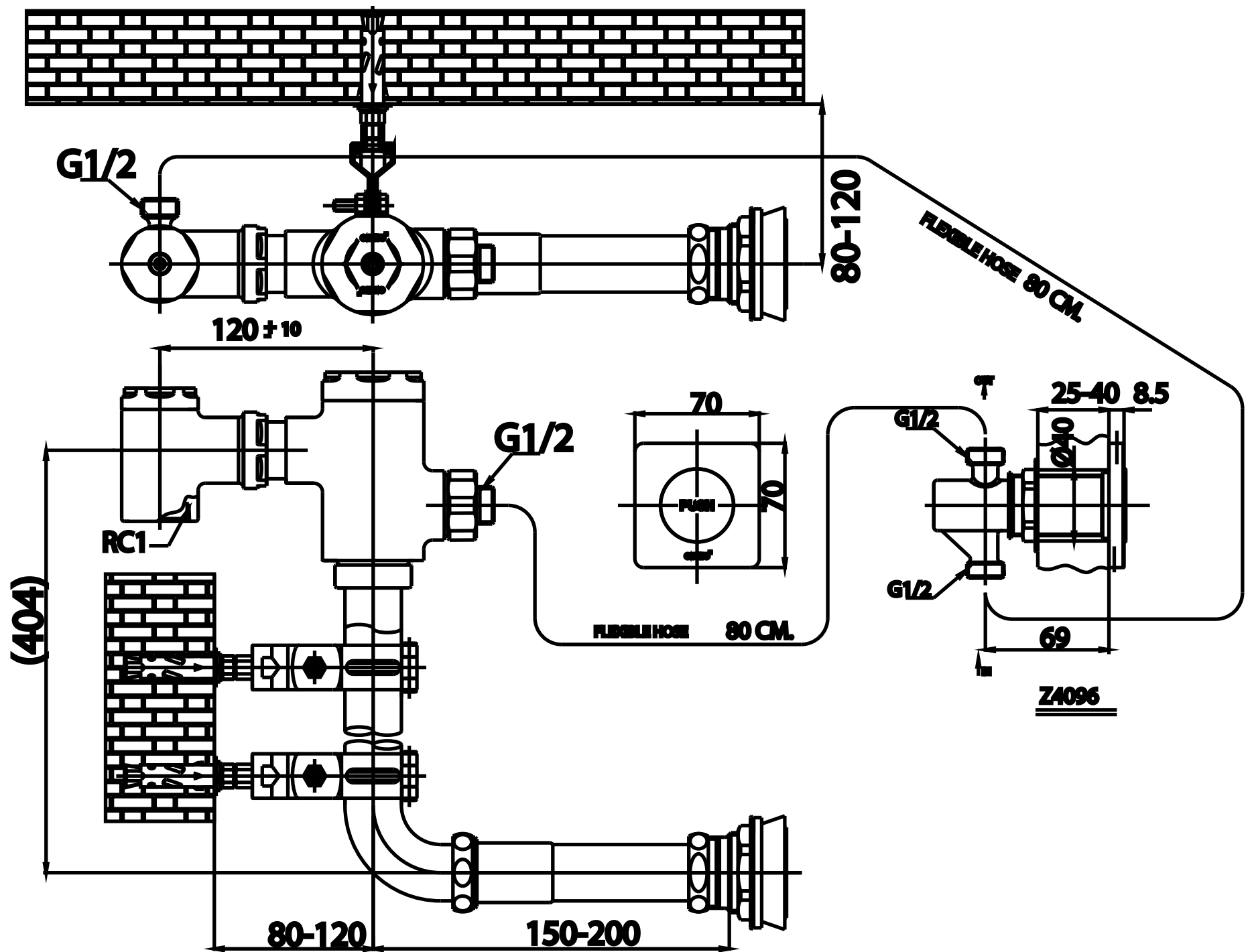
CONCEALED TOILET FLUSH VALVE CT456NL
